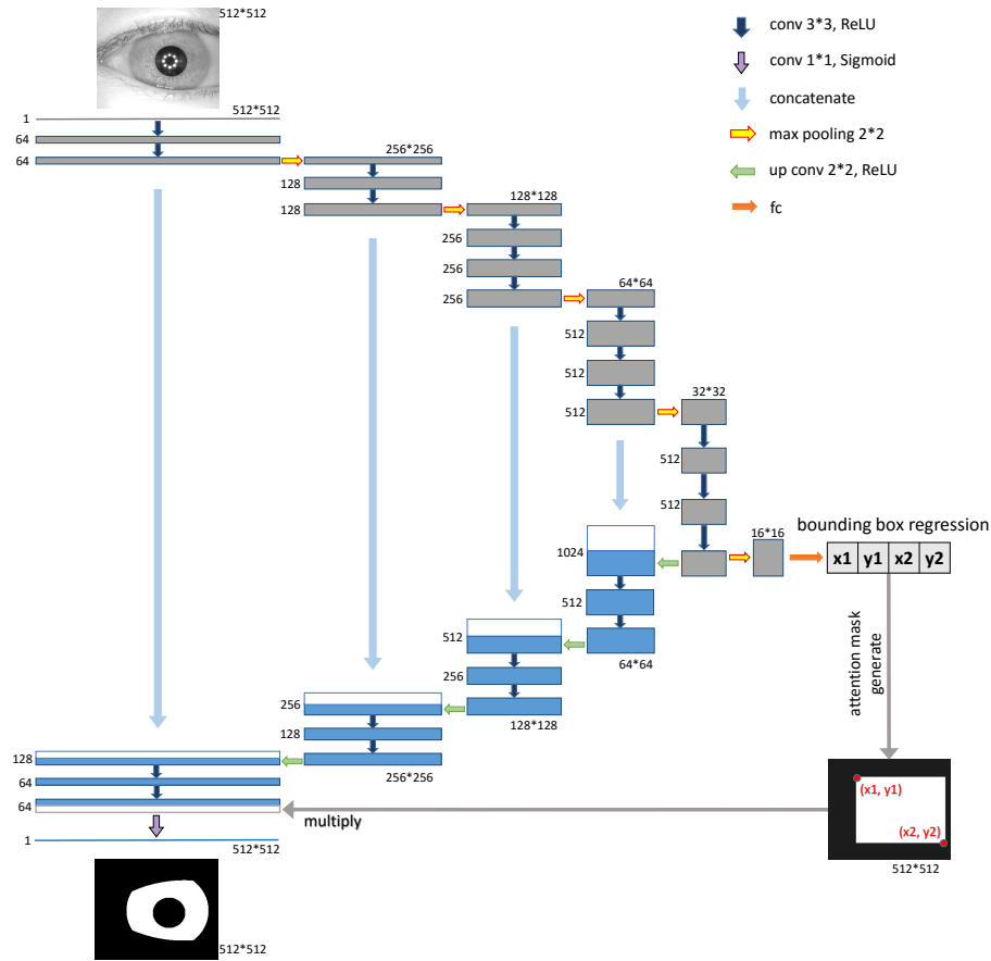
Figure 2: ATT-UNet architecture. All the boxes correspond to multi-channel feature map. The contracting path of ATT-UNet use the same architecture as VGG16( without fc top ). The gray-colored part of ATT-UNet is also act as the bounding box regression model and is used for attention mask generation. The generated attention mask is merged back to ATT-UNet and make our model focus on the segmentation of iris region.
