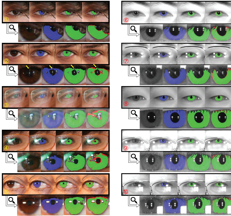
Figure 7: Some challenging samples and their segmentation results are selected and displayed from two datasets. The first columns of both side are original iris images. The second and the third column respectively display the groundtruths (marked in blue) and segmentation predictions (marked in green). The false segmented pixels are labeled as red color in fourth column. All the images are zoomed in for detail.
