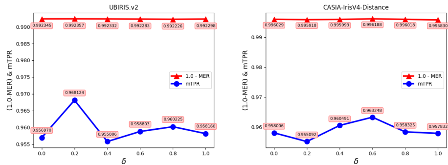
Figure 4: The MER & mTPR metrics of the segmentation results under different soft attention weight for the UBIRIS.v2 and CASIA-IrisV4-Distance datasets. For better display, we use (1.0 - MER) instead.
