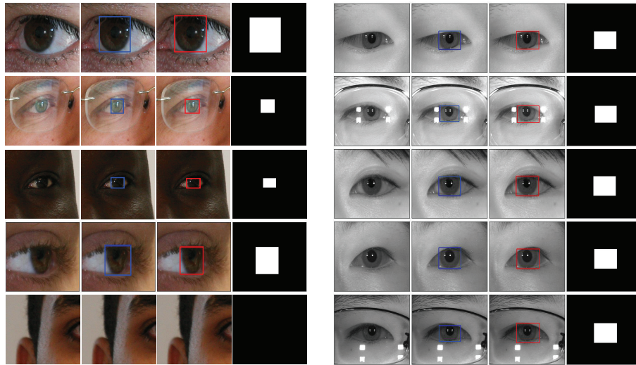
Figure 3: Examples of attention mask generation results. The left part is example results from UBIRIS.v2 and the right part is from CASIA-IrisV4-Distance. The first column of each part is original iris images from each dataset, and the second column is the iris region bounding boxes given by finding max contour on segmentation masks. The example bounding boxes predicted by gray part of the proposed ATT-UNet are shown in the third column. The fourth column is examples of generated attention mask according to coordinates of bounding box, following the setting of Equation(2). For better locating iris region, we expand the predicted attention rectangles by 5 pixels.
